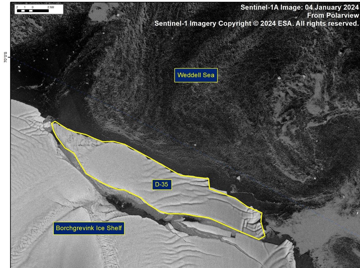
Figure 1: SENTINEL-1 image of iceberg D-35 from January 4, 2024.
